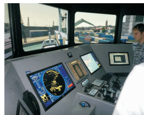
NAUTIS class A Full Mission Bridge Simulator, NAUTIS Class B DP Simulator, new ECDIS Simulator classroom
